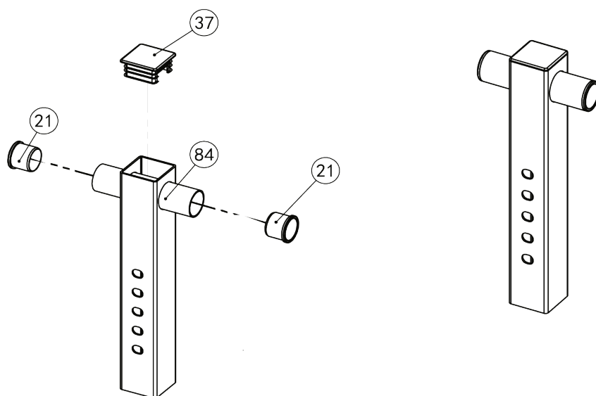
Knee Anchor Adjust Tube Assembly Part-66 1PC/SET
