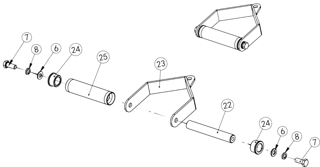
Single Metal Handle-83 2PC/SET
