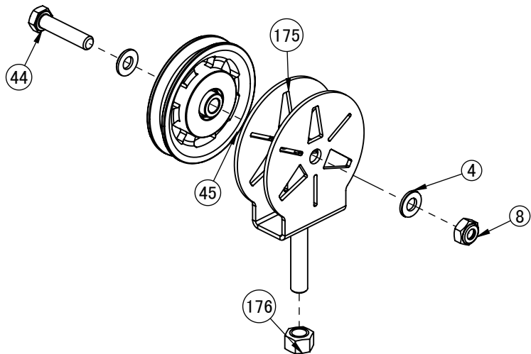
Pulley Frame
