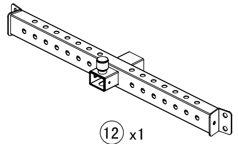
Leg Press Connection Frame
